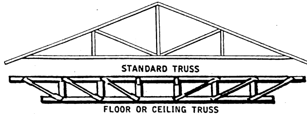
FLOOR OR CEILING TRUSS
