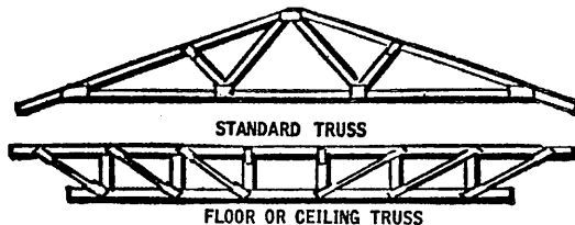
FLOOR OR CEILING TRUSS
